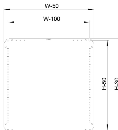
Mounting plate
